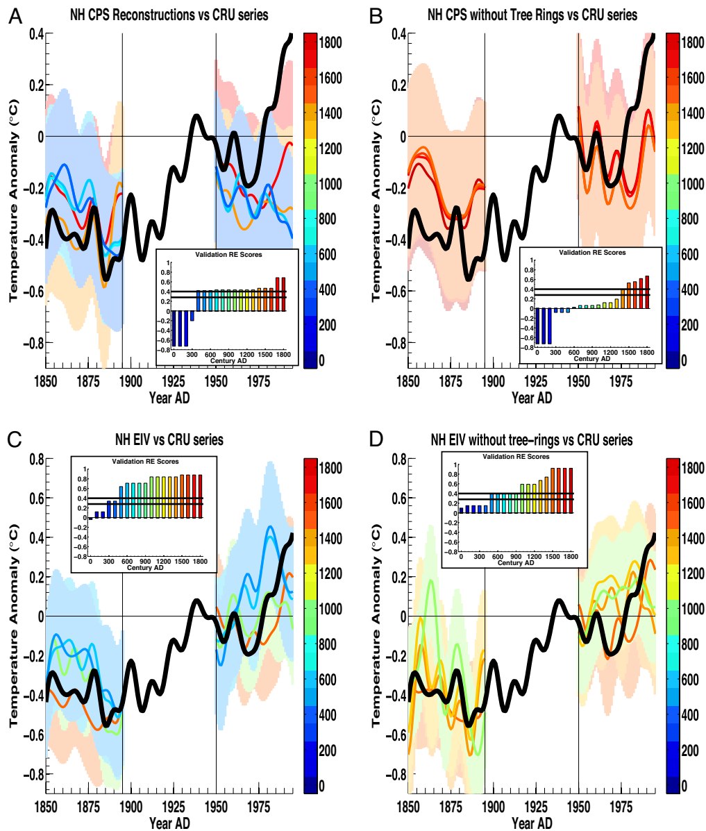
Fig. 2. Comparison of CPS: hemisphere screened ( A ); “no dendro” ( B ); and EIV full global ( C ) and “no dendro” ( D ). NH reconstructions (colored curves; 95% confidence intervals shown by lightly shaded regions of similar color) with decadal smoothed CRU NH land mean series (thick black curve). Reconstructions are shown over late (A.D. 1950–1995) and early (A.D. 1850–1895) validation intervals corresponding to early (A.D. 1850–1949) and late (1896–1995) calibration experiments respectively. RE validation scores are shown ( insets ) as a function of the starting date of the network along with 90% and 95% significance levels based on Monte Carlo experiments. Only reconstructions that passed validation are shown. Color bar indicates network starting dates.
