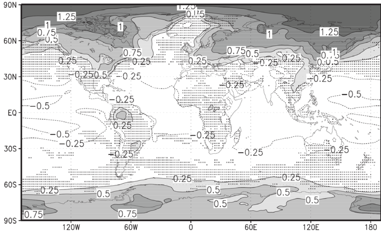
Figure 4. All-model ensemble annual average surface air temperature differences (K) for G1 minus the control run, averaged over years 11-50 of the simulation. Stippling indicates where fewer than 75% of the models (9 out of 12) agree on the sign of the difference. (from Figure 2 from ref 25.)
