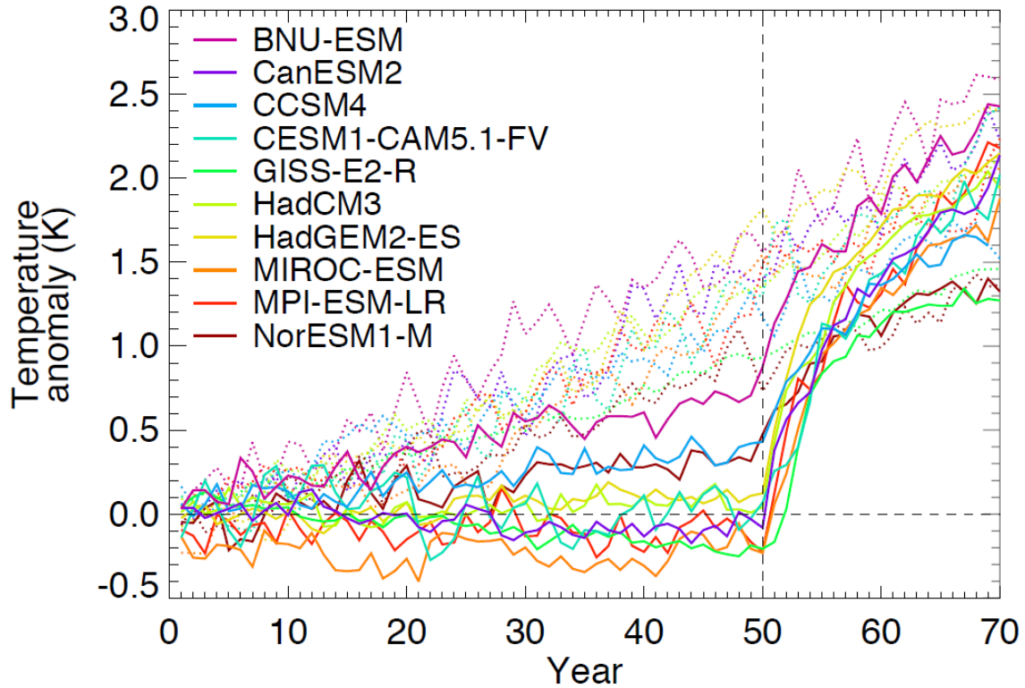
Figure 3. Evolution of annual mean anomaly of global mean near-surface air temperature (K) in the G2 simulations (solid lines) with respect to the long-term mean from each model's control simulation. Time series from corresponding 1% CO 2 /year increase simulations are also shown (dotted lines). The termination of geoengineering in the G2 simulations is indicated by the dashed vertical line. (Figure 1 from ref. 24. See that reference for climate model abbreviations and details.)
