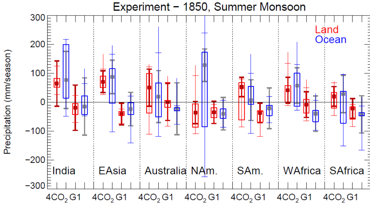
Figure 7. Summer monsoon change of precipitation for 4xCO 2 and G1 with regard to 1850 (control) conditions. Results are for land (red – 1 st and 3 rd column for each region) and ocean (blue – 2 nd and 4 th column for each region) and for different regions (Figure 6). The multi-model range is illustrated by a vertical line, the 25th and 75th percentile of multi-model results are given as a colored box, and the 5th and 95th percentile are horizontal bars. In addition, the multi-model median is shown as solid symbols and the interannual variability of each experiment, represented by the median standard deviation of seasonal averages for each model, is shown as error bars pointing off the median of the multi-model results (dark red for land and grey for ocean). The two left whisker plots for each region are the 4xCO 2 statistics, and the two rightmost whisker plots are for G1. (from Figure 14 from ref. 30.)
