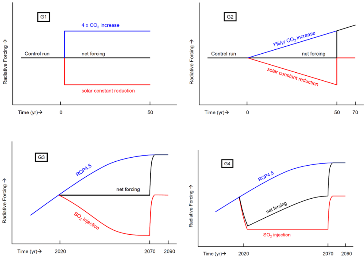
Figure 2. The four GeoMIP experiments, described in Table 1. G1: The experiment is started from a control run. The instantaneous quadrupling of CO 2 concentration from preindustrial levels is balanced by a reduction in the solar constant until year 50. G2: The experiment is started from a control run. The positive radiative forcing of an increase in CO 2 concentration of 1% per year is balanced by a decrease in the solar constant until year 50. G3: The experiment approximately balances the positive radiative forcing from the RCP4.5 scenario by an injection of SO 2 or sulfate aerosols into the tropical lower stratosphere. G4: This experiment is based on the RCP4.5 scenario, where immediate negative radiative forcing is produced by an injection of SO 2 into the tropical lower stratosphere at a rate of 5 Tg per year. (Figures 1-4 from ref. 22.)
