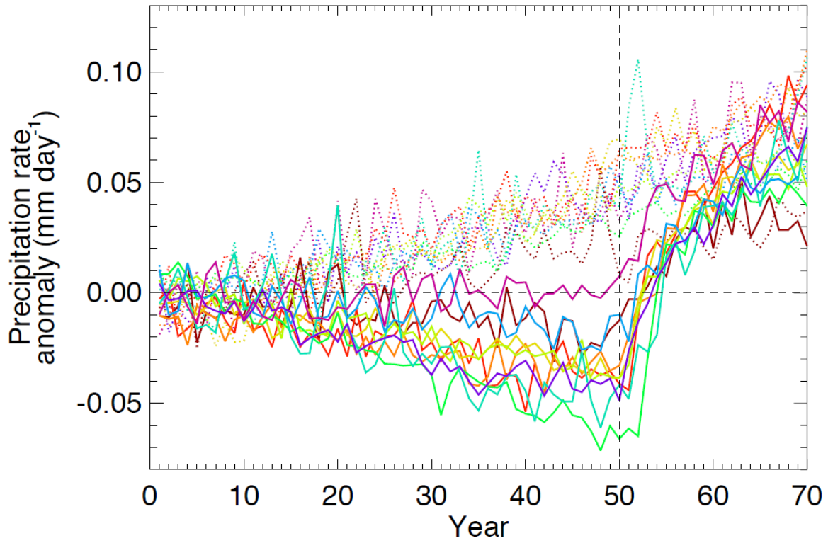
Figure 5. As in Figure 3 but for the anomaly in global mean precipitation rate (mm day -1 ). (Figure 2 from ref. 24. See that reference for climate model abbreviations and details.)
