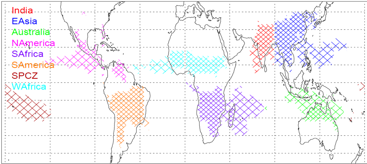
Figure 6. Monsoonal regions (different colors) over land (small hashes) and ocean (large hashes), derived from the Global Precipitation Climatology Project (GPCP) dataset 58 , covering the years 1979 to 2010, and using criteria described in ref. 26. The North and South American monsoon are defined here as the American monsoon North and South of the equator, respectively. (Figure 6 from ref. 30.)
