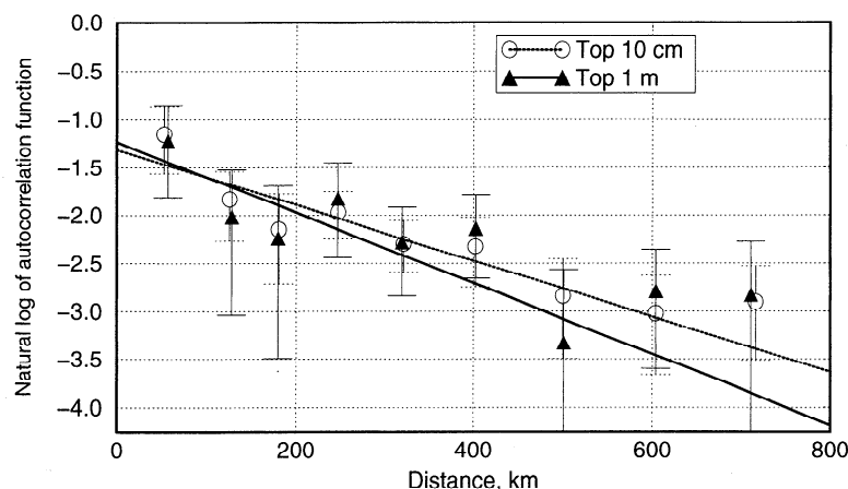
Figure 11. Same as Figure 4 except using 42 stations from Mongolia.
