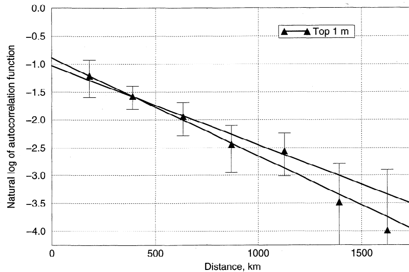
Figure 9. Same as Figure 4 except using 50 stations from Russia, and only the top 1 m soil moisture data.
