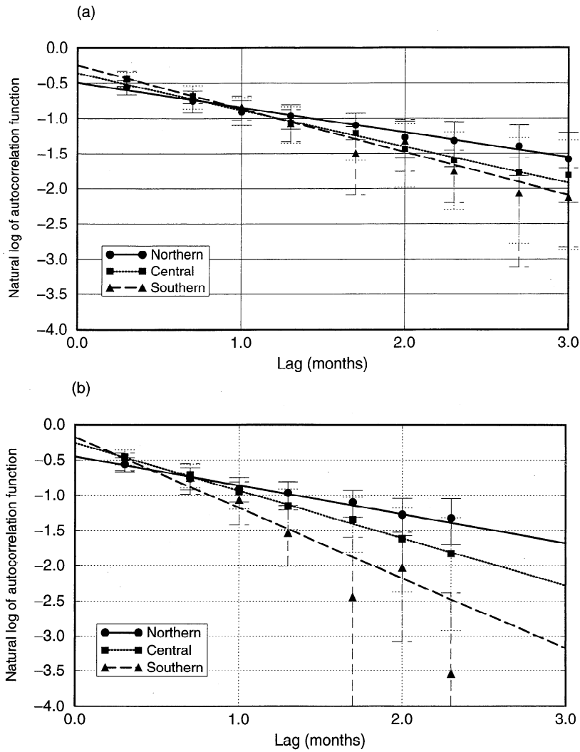
Figure 8. Similar to Figure 3, except each line represents data only from stations located within each designated area shown in Figure 2 for the top 1 m: (a) all seasons and (b) no winter.
