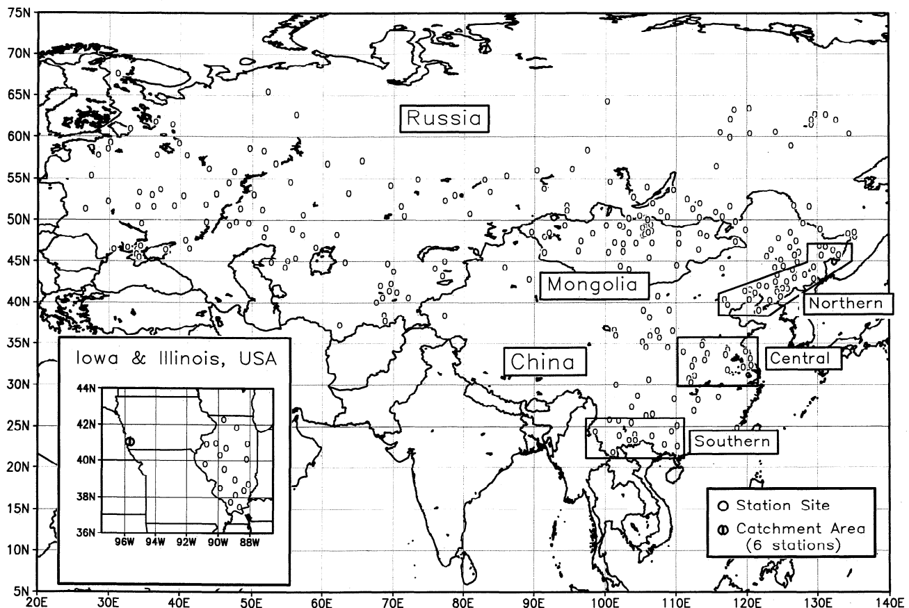
Figure 2. Stations used in this analysis. The three boxed areas in China, northern, central, and southern, were used for specific regional study of the temporal scales, discussed in section 4.1.
