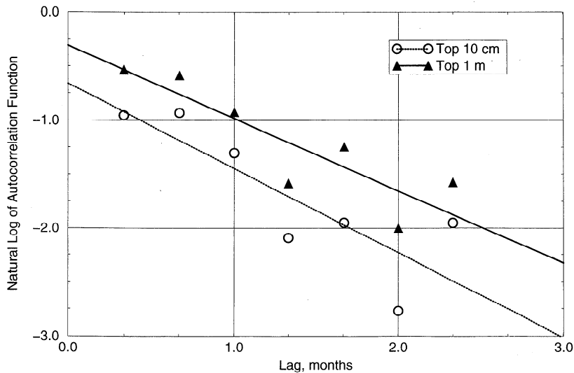
Figure 7. Same as Figure 3 except using the six soil moisture records from Iowa. Due to the low number of records, the 95% confidence intervals were omitted.
