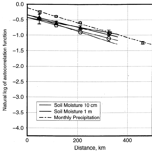
Figure 4. Spatial correlation points and best fit line for Illinois, with mean spatial autocorrelation values for each distance bin for the 17 soil moisture stations in Illinois. Also shown are similar points for monthly precipitation for 87 stations in the Illinois area. All error bars denote the 95% confidence interval about each mean point.
