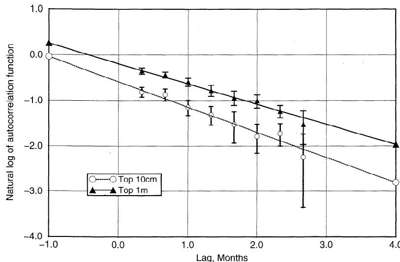
Figure 3. Mean temporal autocorrelation values and best fit line, for the 17 stations in Illinois. The error bars denote the 95% confidence interval about each mean point.
