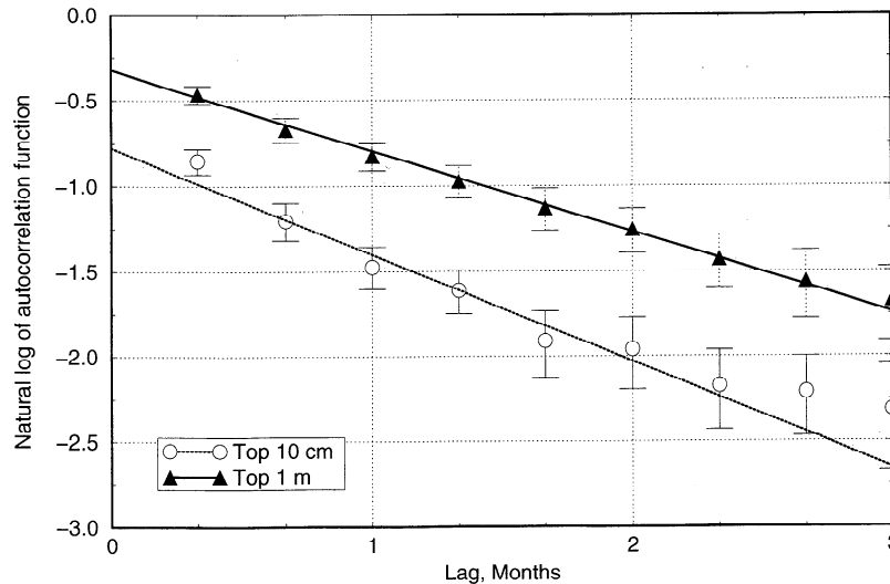
Figure 5. Same as Figure 3 except using 78 stations from China.
