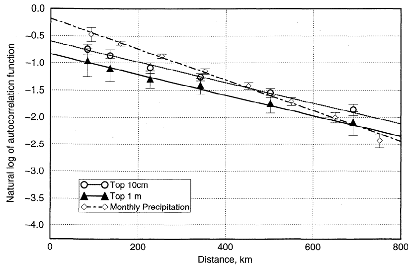
Figure 10. Same as Figure 4, except using 78 soil moisture and 275 precipitation stations from China.
