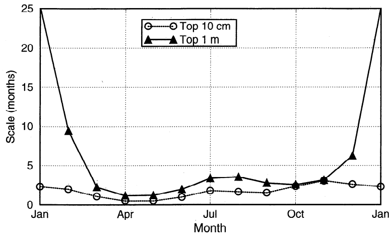
Figure 12. Seasonal temporal scale for Illinois. See text for explanation of how the scales were calculated.
