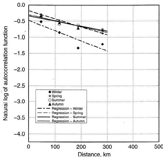
Figure 13. Same as Figure 4, except each line represents data only from those months corresponding to the designated season (winter is December, January, February; spring is March, April, May, etc.). Analysis shown is only for the top 1 m. Regression lines were determined using the least squares method.
