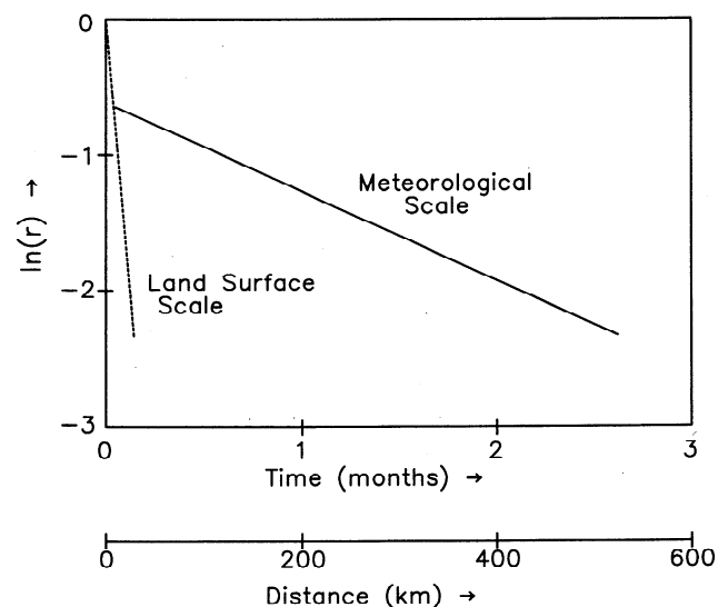
Figure 1. Schematic diagram of hydrological and meteorological scales of soil moisture variations. R is the autocorrelation function. The scales are determined separately by the two terms from (3) for the temporal scale, and from (6) for the spatial scale. Reprinted, with small modifications, from Global Planet. Change , 19, Robock, A., C. A. Schlosser, K. Y. Vinnikov, N. A. Speranskaya, J. K. Entin, and S. Qiu, Evaluation of AMIP soil moisture simulations, 181-208, Copyright (1998), with permission from Elsevier Science.
