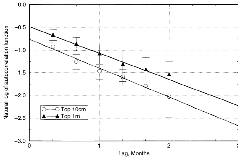
Figure 6. Same as Figure 3 except using 42 stations from Mongolia.
