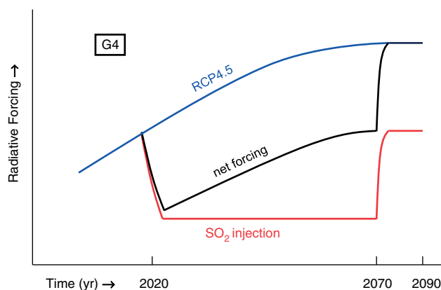
Figure 4. Schematic of experiment G4. This experiment is based on the RCP4.5 scenario, where immediate negative radiative forcing is produced by an injection of SO 2 into the tropical lower stratosphere at a rate of 5 Tg per year.
