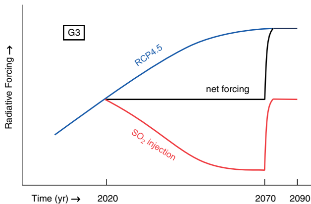
Figure 3. Schematic of experiment G3. The experiment approximately balances the positive radiative forcing from the RCP4.5 scenario by an injection of SO 2 or sulphate aerosols into the tropical lower stratosphere.
