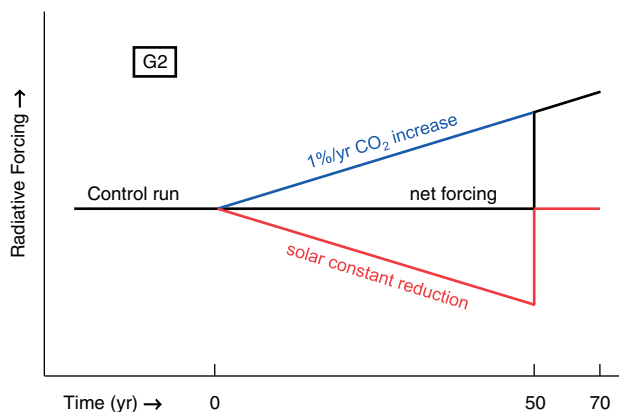
Figure 2. Schematic of experiment G2. The experiment is started from a control run. The positive radiative forcing of an increase in CO 2 concentration of 1% per year is balanced by a decrease in the solar constant until year 50.
