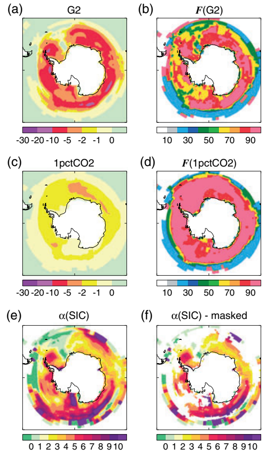
Figure 10. As in Figure 9 but for Antarctica.
