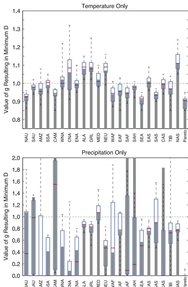
Figure 2. The amount of geoengineering ( g ) that minimizes regional changes ( D , equations (4) and (5) in temperature (top) and precipitation (bottom) for each region ( x -axis). Dashed grey line indicates g = 1 , in which global mean temperature is returned to the preindustrial value. Red lines denote the median response of the 12 models, blue boxes denote 25th and 75th percentiles of model response, and black whiskers indicate the range of model spread. Grey bars show the response for the all-model ensemble mean. Note that ordinates have different scales.
