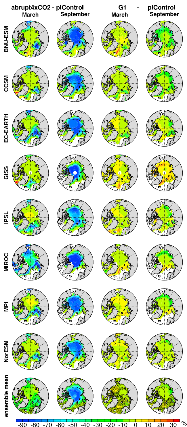
Figure 3. Model simulations of March (maximum sea ice extent) and September (minimum extent) sea ice concentration anomalies (%) for abrupt4xCO2-piControl and G1-piControl for the eight models we analyze here. The ensemble mean has stippling where less than six of eight models agree on sign of change. Figure S2 shows the actual sea ice concentration map for each experiment.
