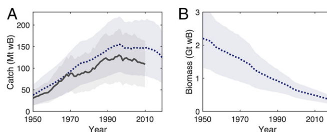
Fig. 1. Prewar trajectories of global fisheries. Simulated (A) annual wild fish catch (megatons wet biomass) and (B) total wild commercially targeted fish biomass (gigatons wet biomass) over 1950 to 2019 from the prewar fisheries baseline using the BOATS model with no fisheries regulation. Shaded areas show the SD for the five parameter ensemble runs, and the dotted lines show the ensemble mean. The fishery and ecosystem state in 2019 are used as initial conditions for the nuclear war scenarios. In A, the gray solid line shows empirical global catches from ref. 33, with uncertainty indicated by the shaded area.
