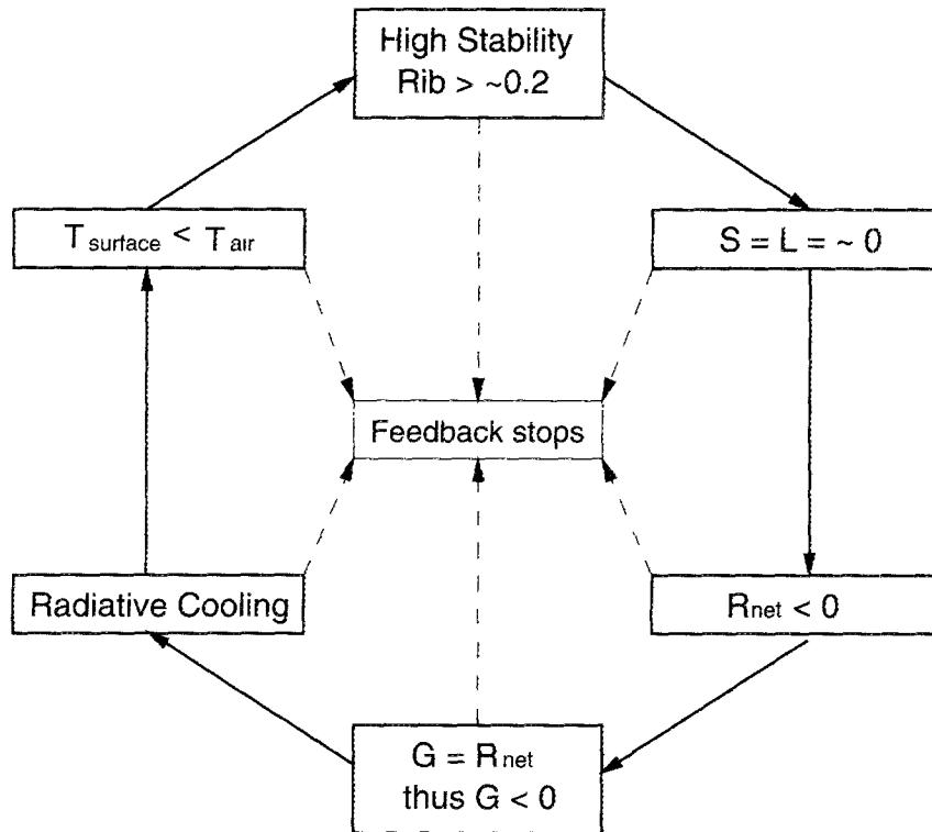
FIG. 8 The stability-induced cooling feedback illustrating a decoupling of surface and atmosphere. Solid arrows indicate that the condition in the box is true, dashed lines indicate that they are false. As the snow surface cools, more energy will later be required for melt to occur. R_{net} , G , S , L , and Ri_b are net radiation, ground heat flux, sensible heat, latent heat, and the bulk Richardson number, respectively.
