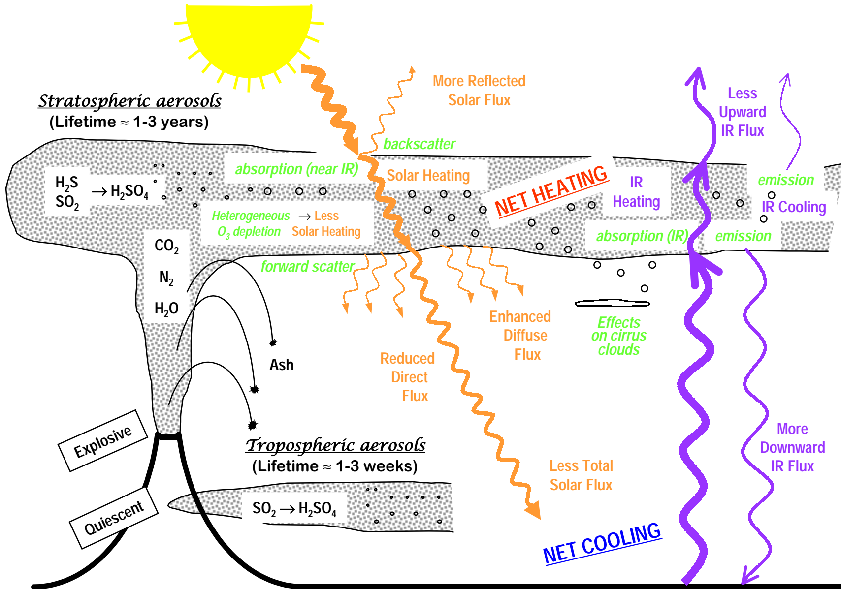
Figure 1 from "Volcanic eruptions and climate" by Alan Robock, Rev. Geophys. , 38, pp. 191-219, 2000.
