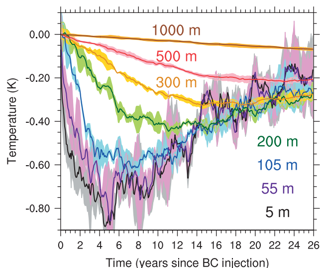
Figure 6. The time evolution of the global average ocean temperature anomaly at various depths is shown. The lines show the monthly average of the experiment ensemble temperatures minus the monthly average of the control ensemble. Shading around each line shows the range of the experiment ensemble runs with respect to the control ensemble average. The horizontal axis shows time in years. The vertical axis shows temperature in K.
