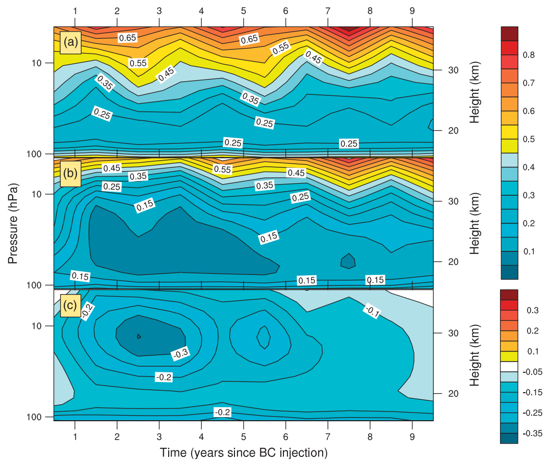
Figure 4. The time evolution of the tropical lower stratospheric vertical wind (mm/s) is shown for (a) the control, (b) the 50 nm experiment, and (c) and the experiment minus the control. Values are ensemble averages for latitudes 22°S to 22°N. The horizontal axis shows time in years. The left vertical axis shows pressure in hPa, and the right shows approximate pressure altitude in km.
