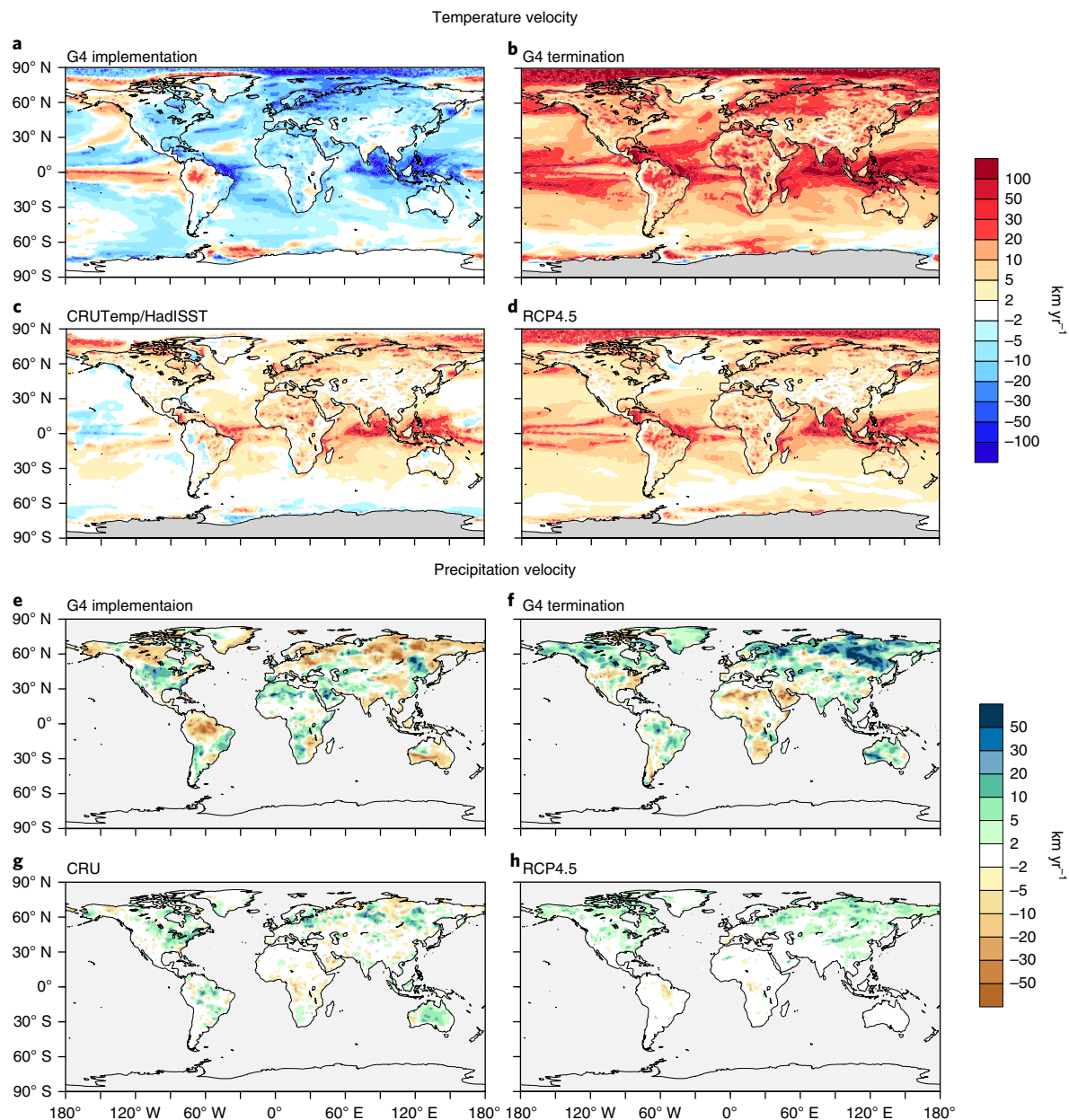
Fig. 2 | Temperature and precipitation velocities for geoengineering implementation, termination, historical climate and RCP4.5. a–d , Temperature velocities. e–h , Precipitation velocities. In c,g , the historical observations for 1960–2014 are shown (CRU TS3.23 for land and HadISST 1.1 for oceans). The speed ( \text{km yr}^{-1} ) of shifting temperature and precipitation isoclines is the same for positive and negative velocities of equal magnitude. The sign of the velocity indicates a trend of local warming (+) or cooling (–) for temperature, and wetting (+) or drying (–) for precipitation. A change of sign between scenarios represents a 180^\circ change in the direction of climate movement (for example, from poleward to equatorward or, in mountain regions, from upslope to downslope).
