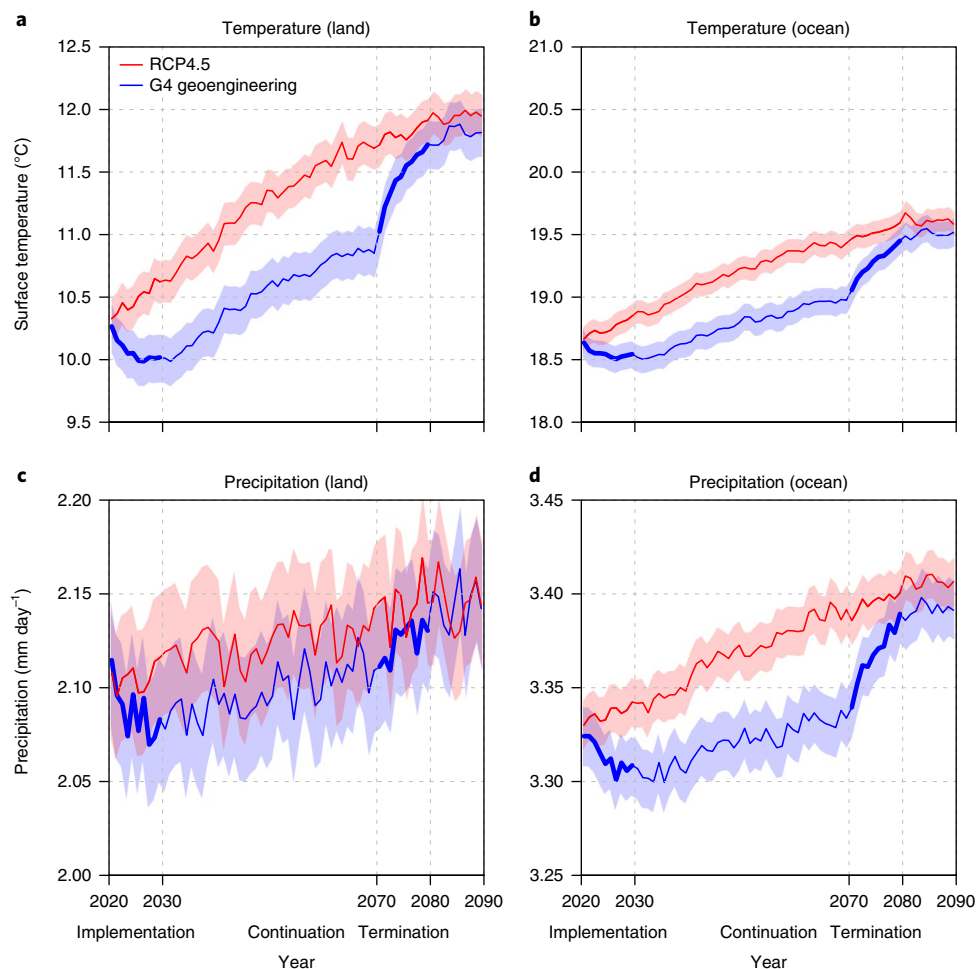
Fig. 1 | Global mean temperature and precipitation for the Geoengineering Model Intercomparison G4 scenario (solar geoengineering) and RCP4.5.
